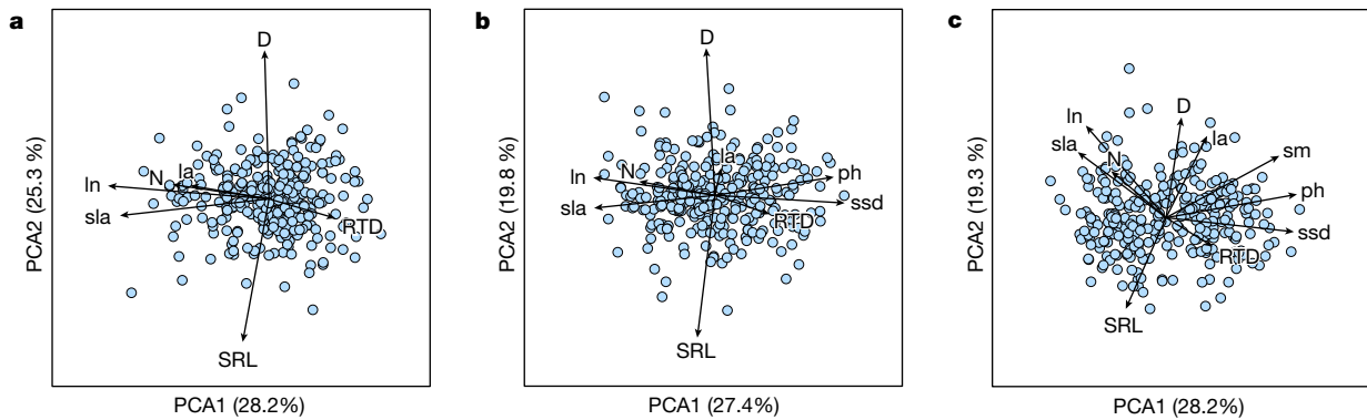
Fig. 1 | PCA of the 301 species analysed in Carmona et al. 1 using differing trait subsets and no varimax rotation. a , Traits strictly related to resource acquisition aboveground (leaf nitrogen content (In), leaf area (la) and specific leaf area (sla)) and belowground (root nitrogen content (N), root tissue density (RTD), root diameter (D) and specific root length (SRL)) show strong
